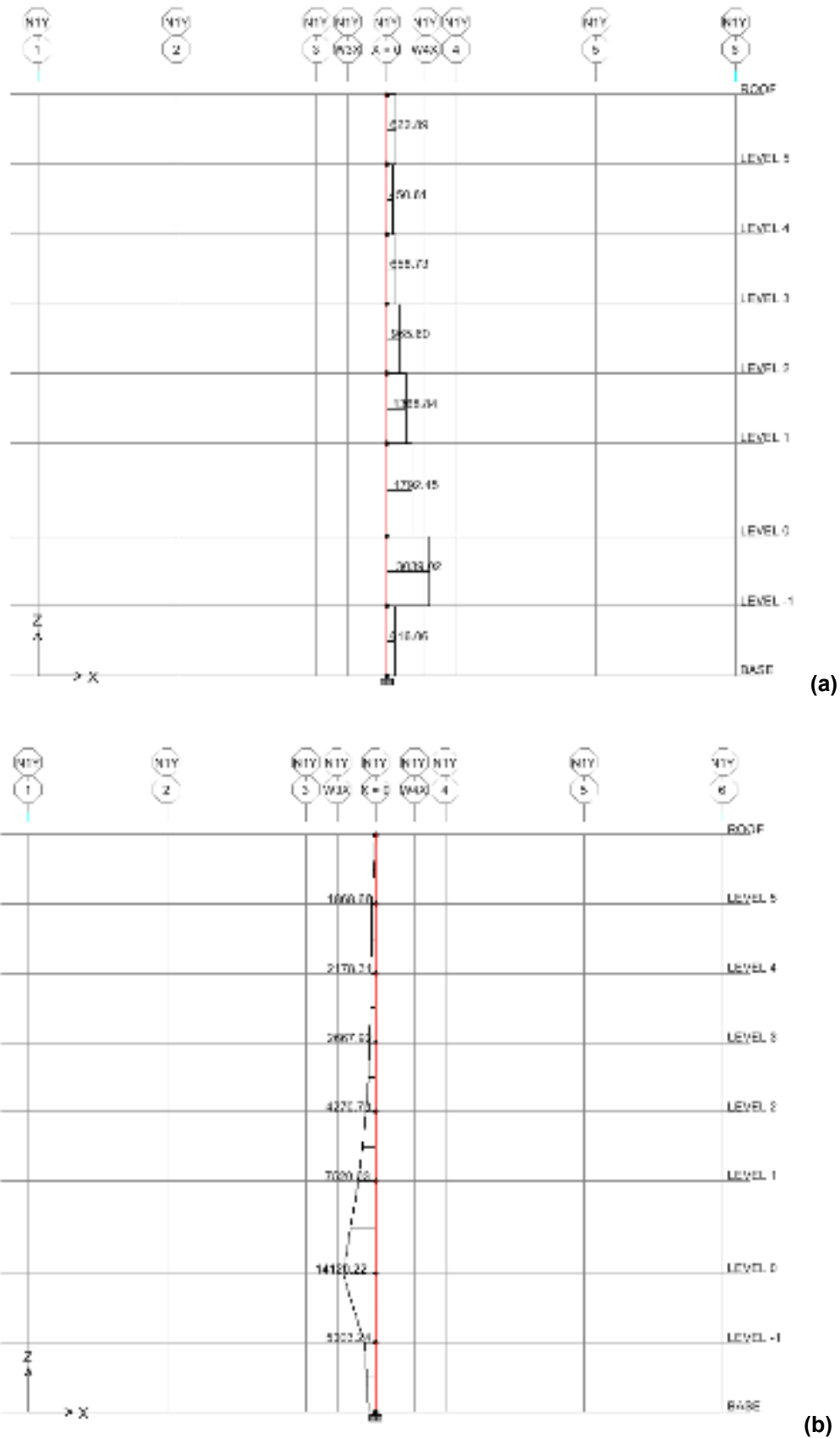
Figure 2.5.8 Shear forces (a) and bending moments (b) for wall N1 (see Figs. 2.1.1 and 2.1.2) in X direction obtained by modal response spectrum analysis.
