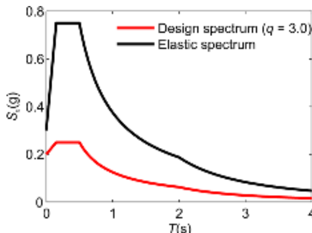
Figure 2.1.3 Elastic and design response spectrum
