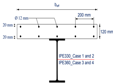
Fig. 5.17.1 Composite beams
