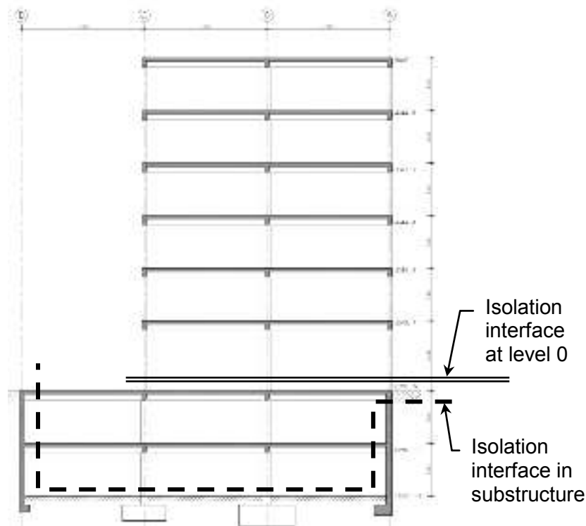
Fig. 6.6.1 Design example
