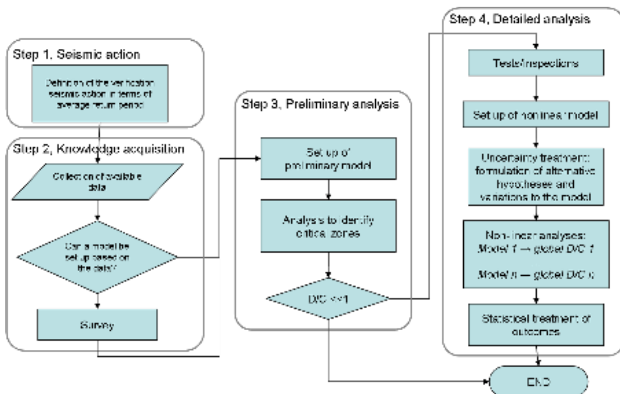
Fig. 7.6.5 Assessment procedure.
