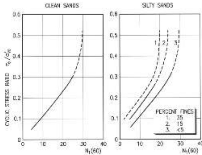
Fig. 4.5.2 Charts giving the liquefaction resistance as function of the corrected blow count for earthquake magnitude 7.5
