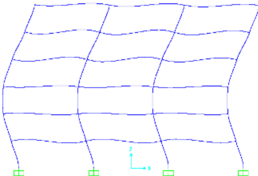
Fig. 5.10.4 Deformed shape in vibration mode 2
