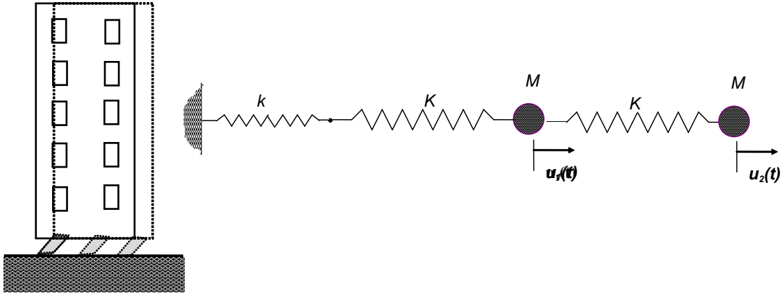
Fig. 6.2.2 Simple model of a building with isolation
