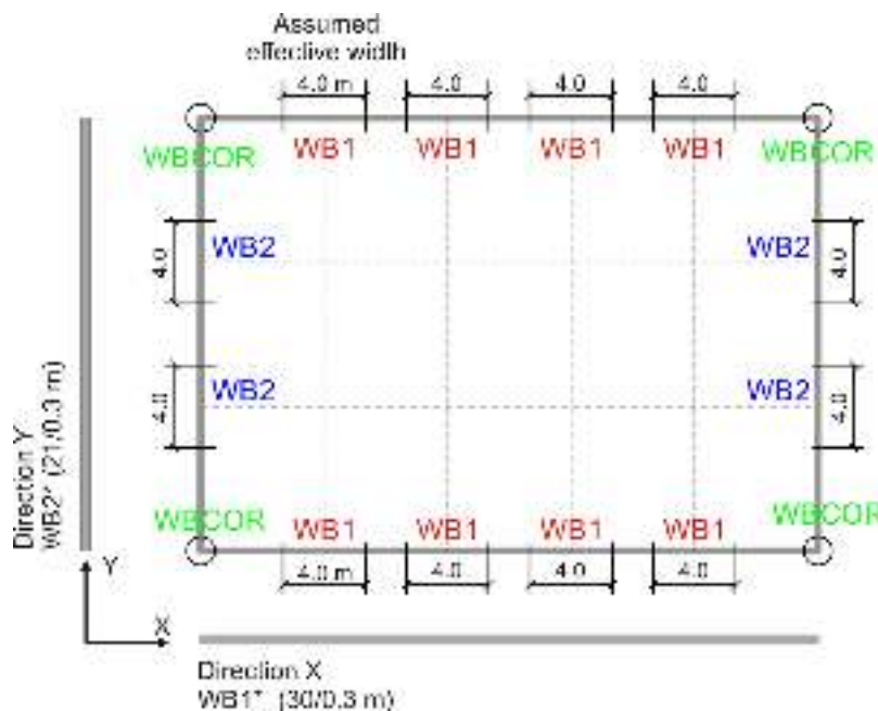
Figure 2.2.3 Modelling the peripheral walls
