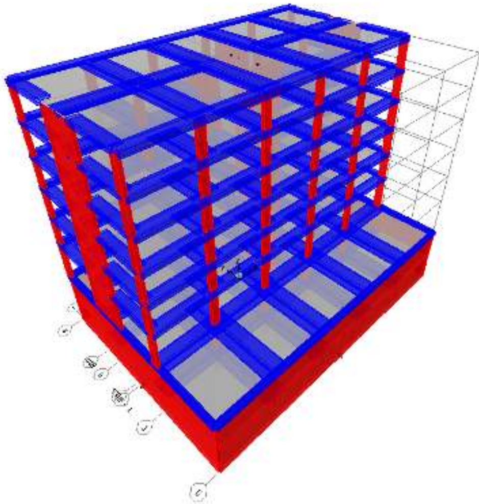
Figure 2.2.1 Structural model
