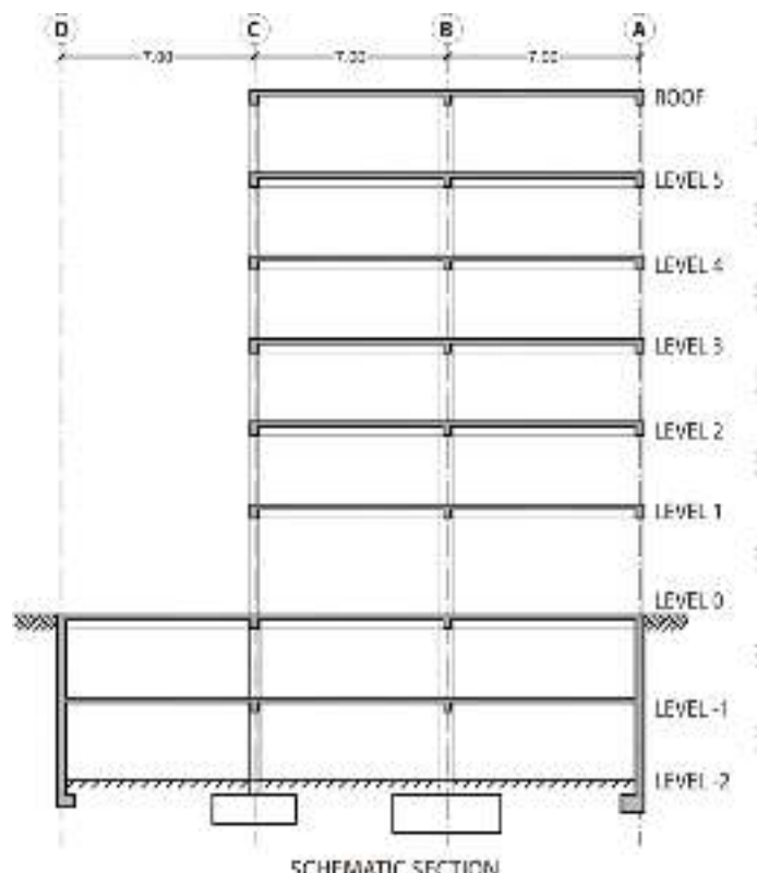
Figure 2.1.2 Schematic cross-section of the building
