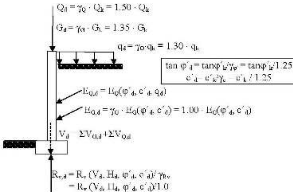
Fig. 4.3.4 Design approach DA-3
