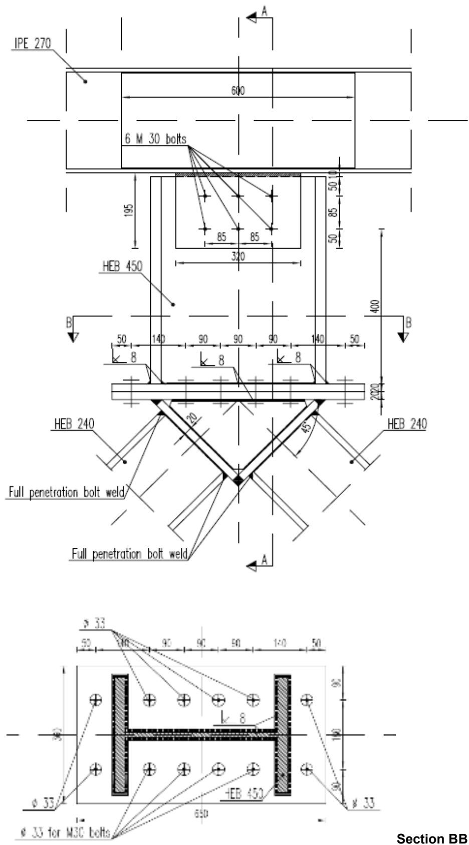
Fig. 5.24.2 View of link in elevation. Section BB: plan view of link base plate
