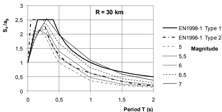
Fig. 1.2.6 Recommended spectral shapes for Type and Type 2 seismic action in EN 1998-1 and illustration of the effect of Magnitude on normalised spectral shape (rock ground conditions)
